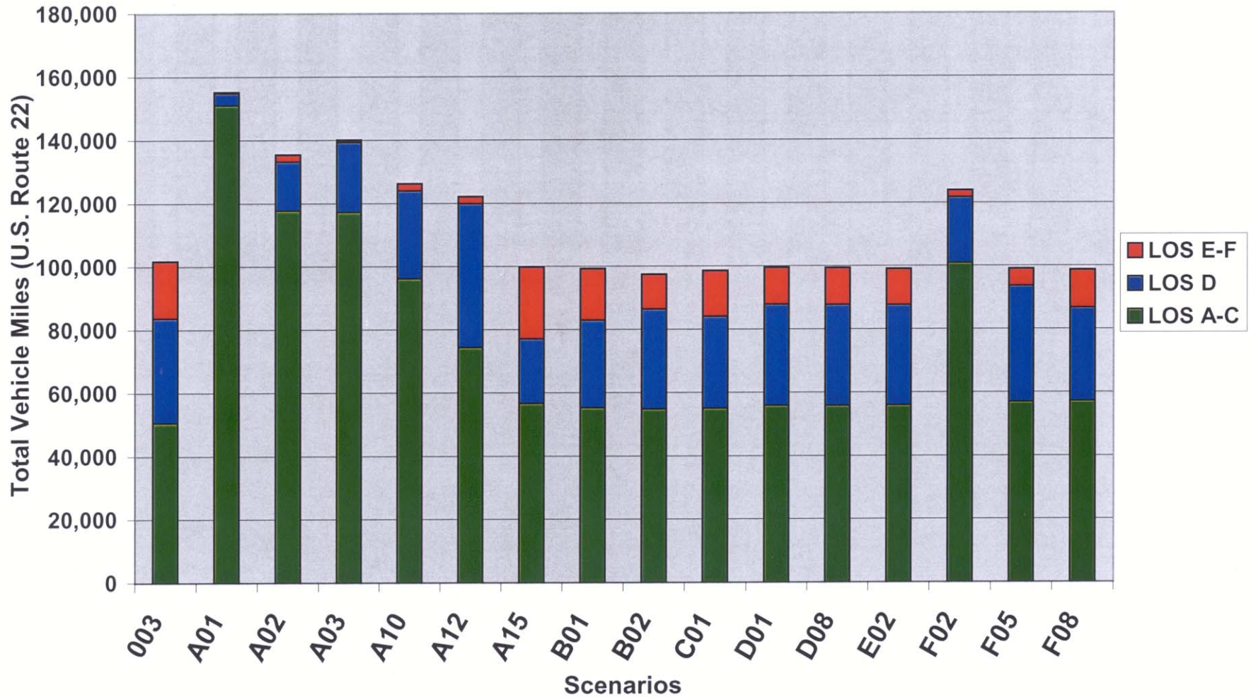
CHART 1 - U.S. Route 22 Comparison of Level of Service by Scenario 2020 PM Peak Hour
